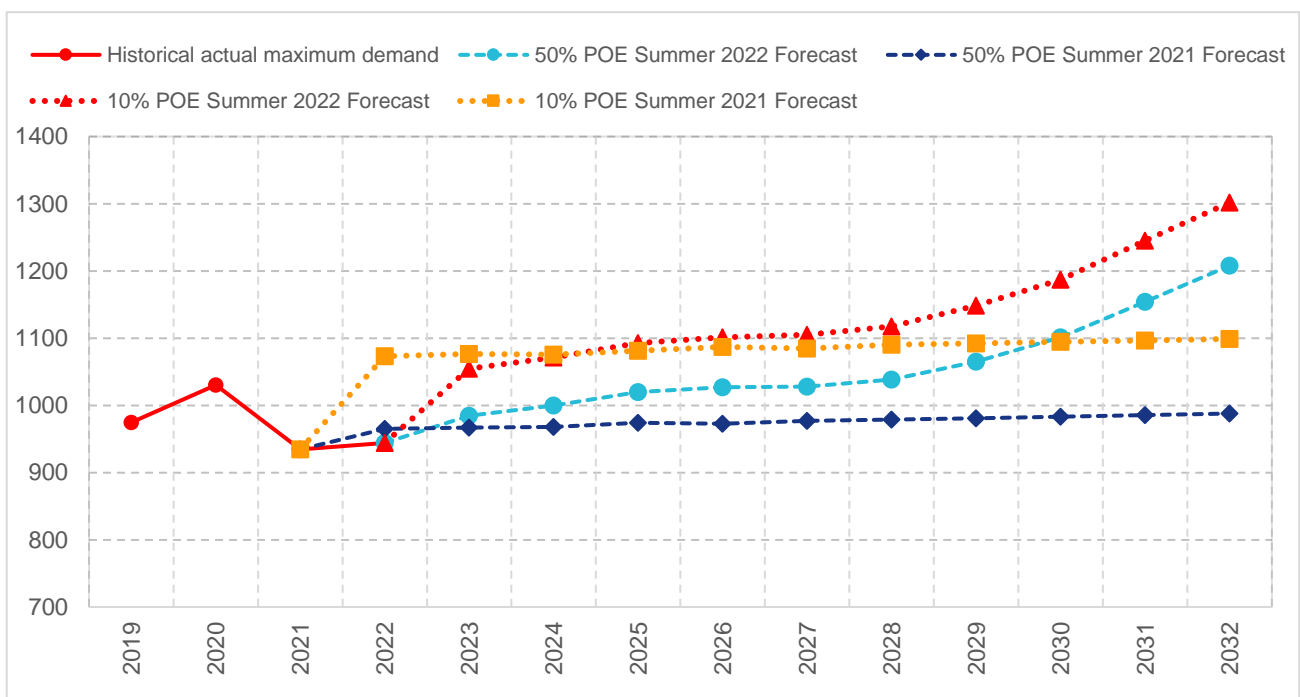
Figure 4-1: Jemena network maximum demand forecast comparison
