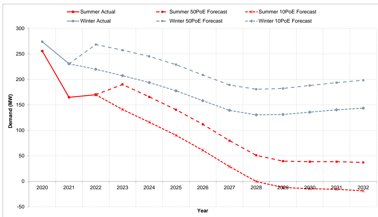
Figure 2: JEN historical and total minimum demand forecast
