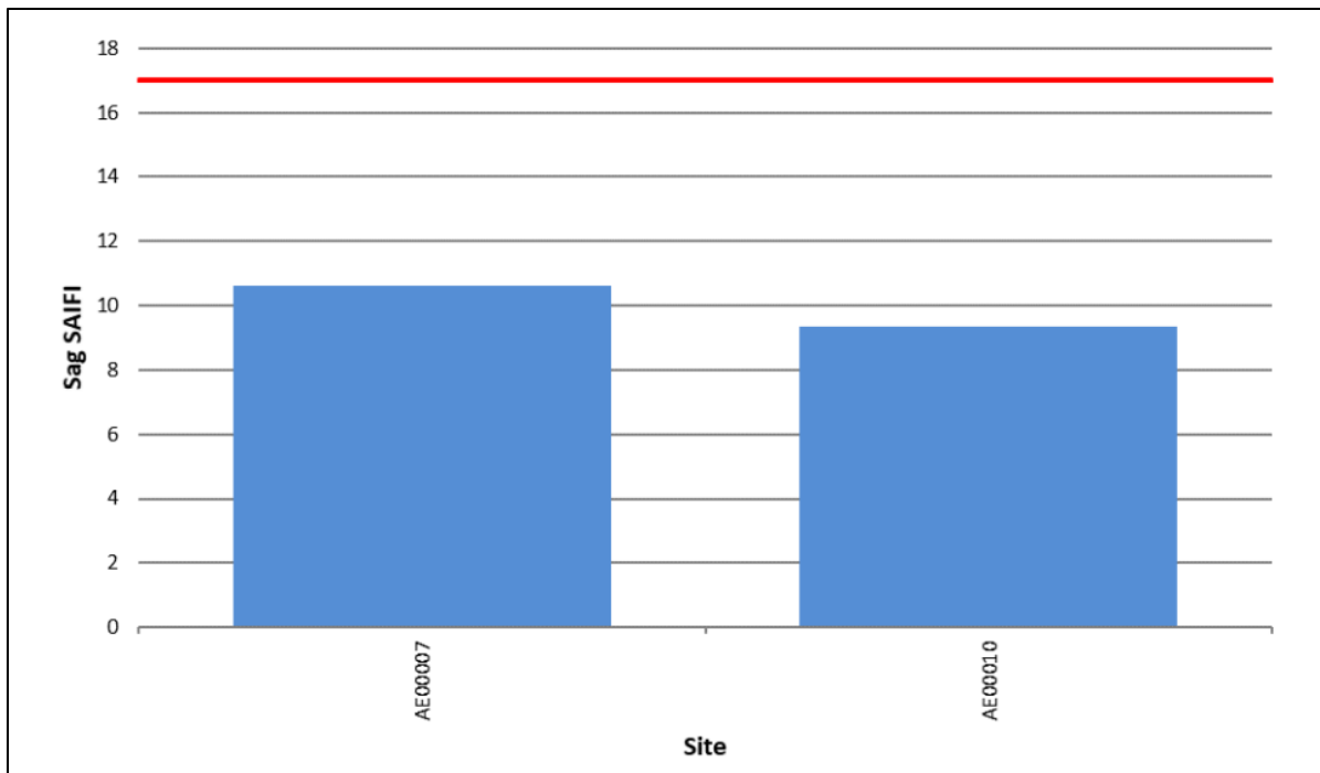
Figure 3-7: Voltage sag performance – 6.6 kV site
