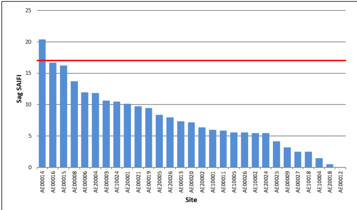
Figure 3-6: Voltage sag performance – 22 kV and 11 kV sites
