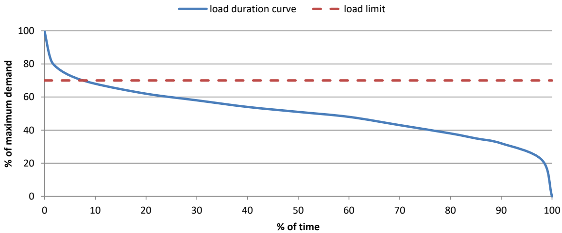
Figure 2-13: Load duration curve and import load limit relationship
