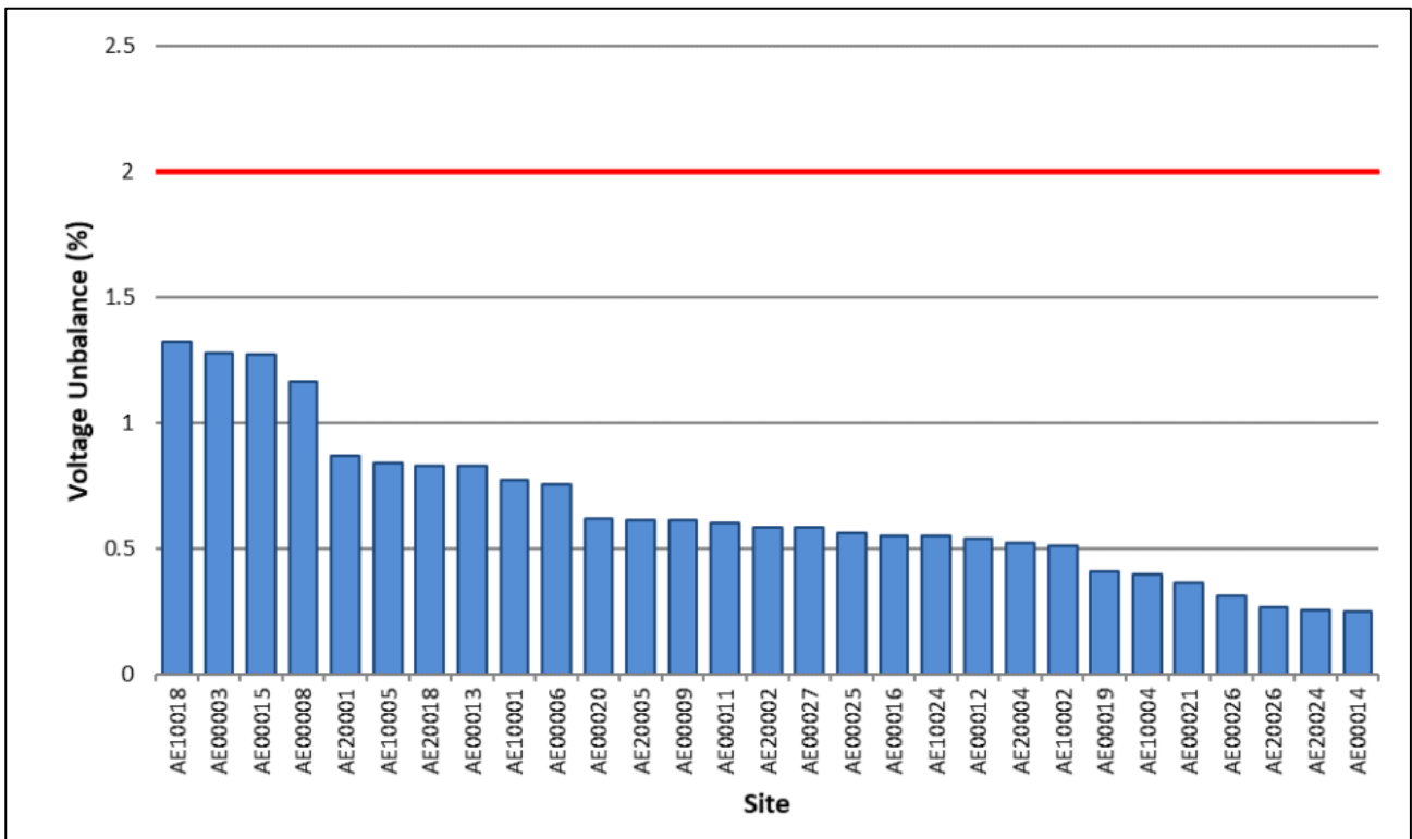
Figure 3-10: Voltage unbalance (negative sequence voltage) – 22 kV and 11 kV sites
