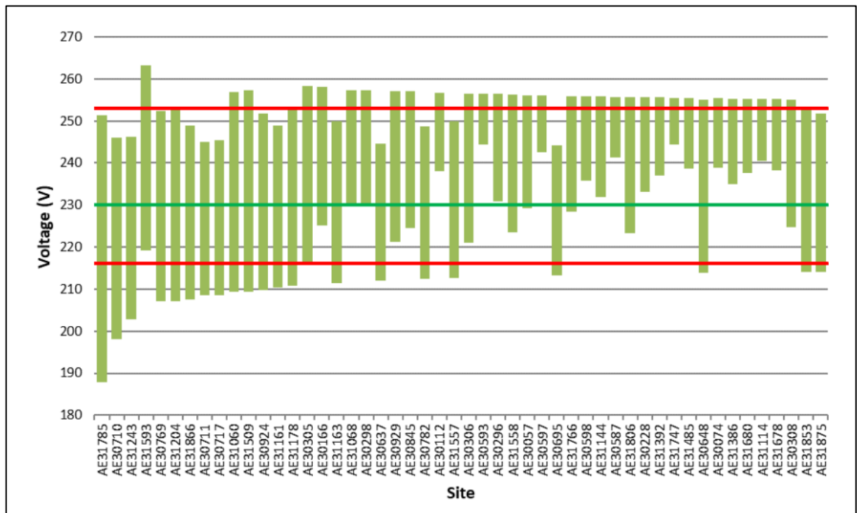
Figure 3-5: Steady-state voltage performance – LV sites (worst 50)
