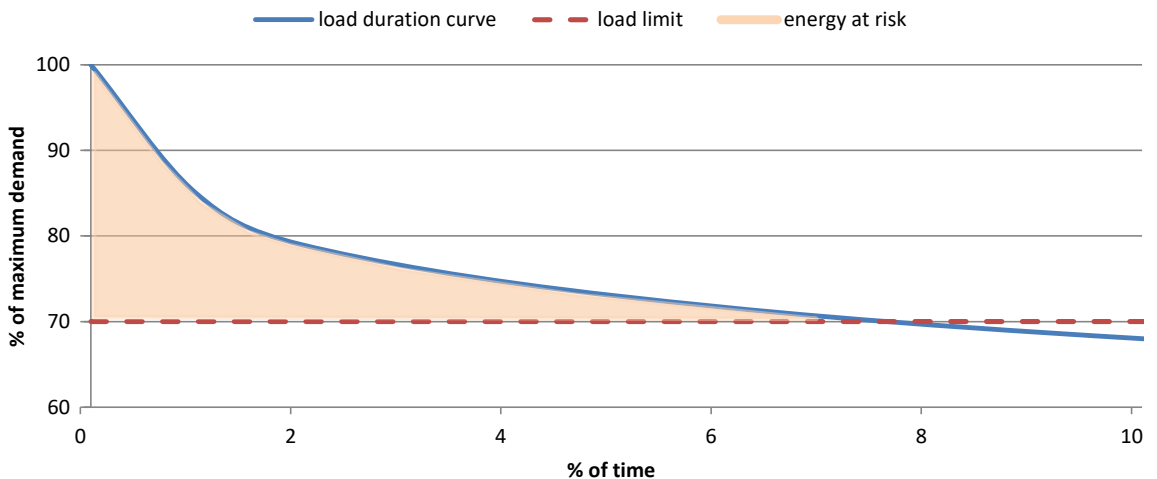
Figure 2-14: Energy-at-risk calculation for the area of the load duration curve above the import load limit
