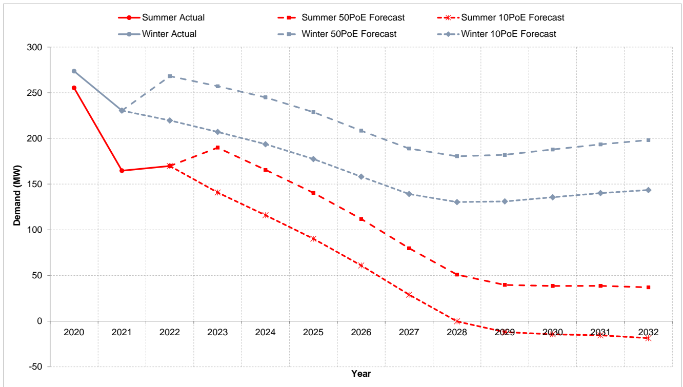
Figure 4-4: Jemena's historical and total minimum demand forecast
