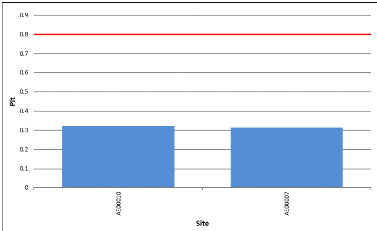
Figure 3-16: 6.6 kV Voltage flicker levels – PIt distribution
