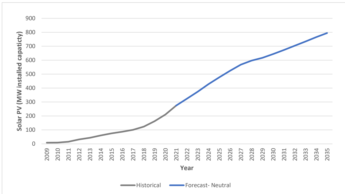
Figure 2-5: Cumulative capacity of installed solar PV systems within Jemena’s supply area
