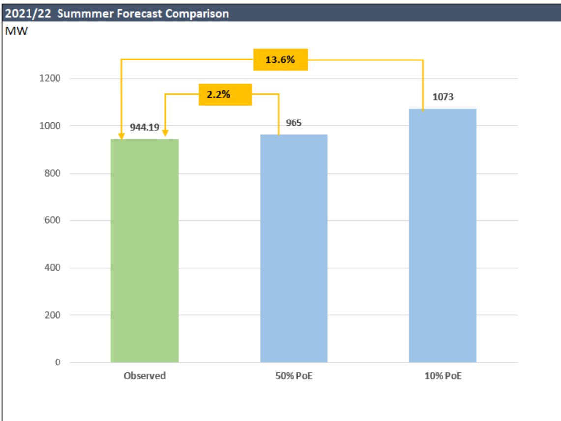
Figure 4-5: JEN Observed Maximum Demand 2021/22
