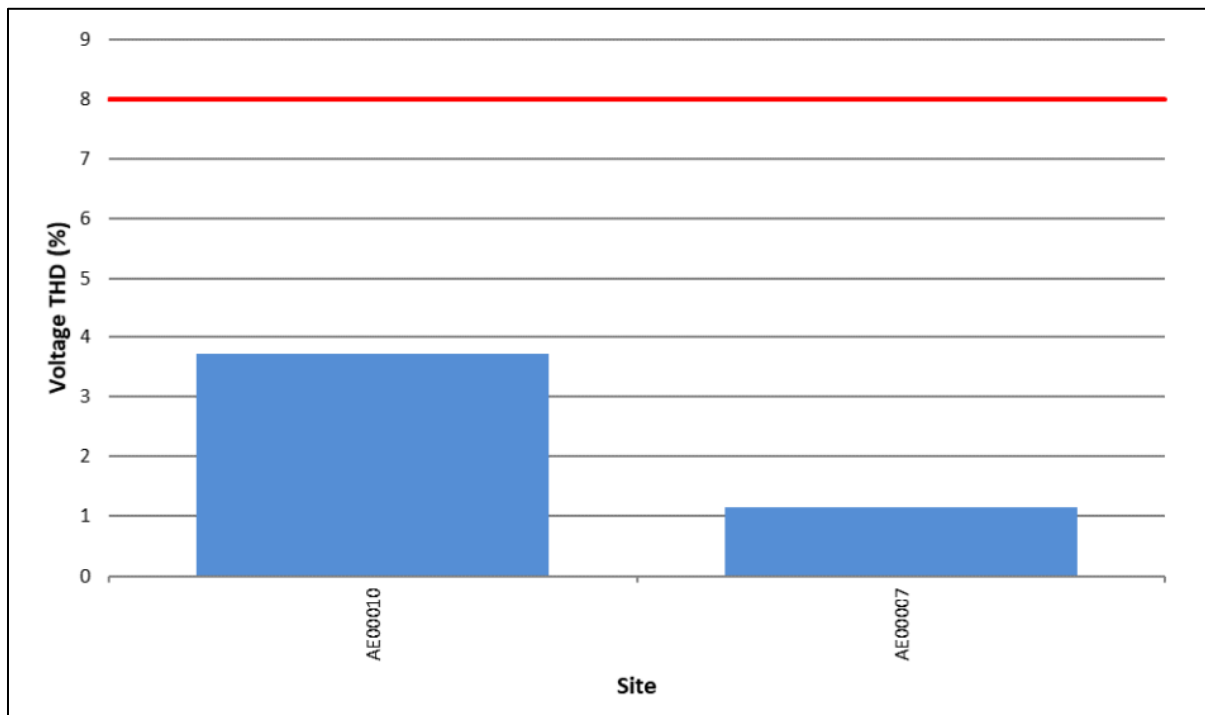
Figure 3-9: Harmonic distortion levels – 6.6 kV sites
