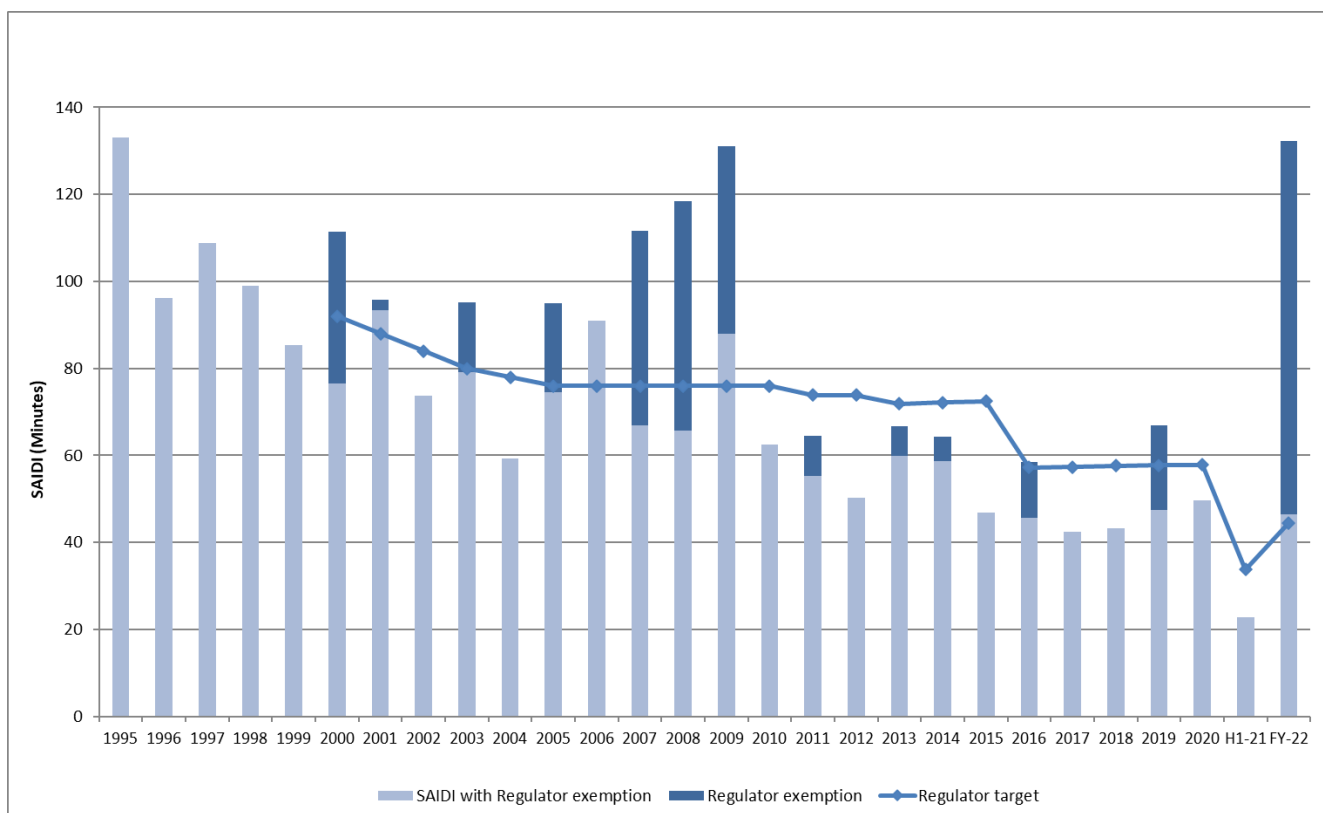
Figure 3-1: Historical unplanned SAIDI network performance (CY 1995-FY2022)
