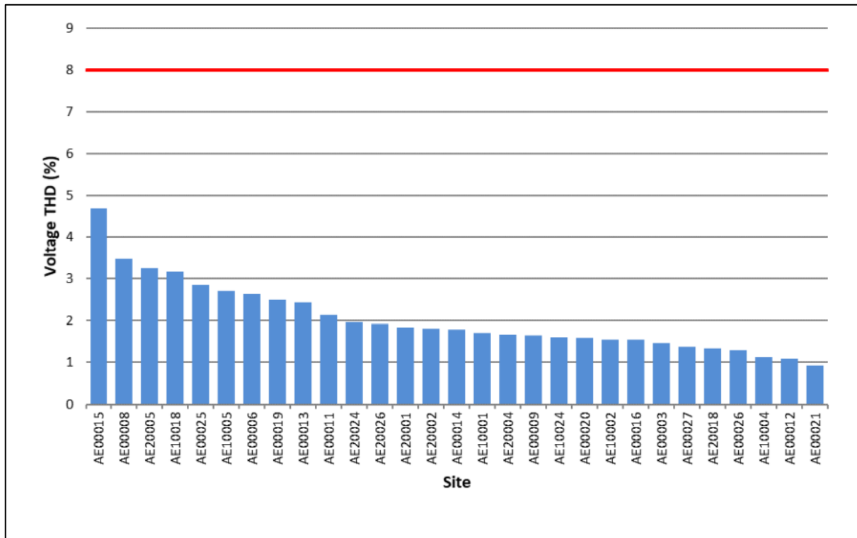
Figure 3-8: Harmonic distortion levels – 22 kV and 11 kV sites
