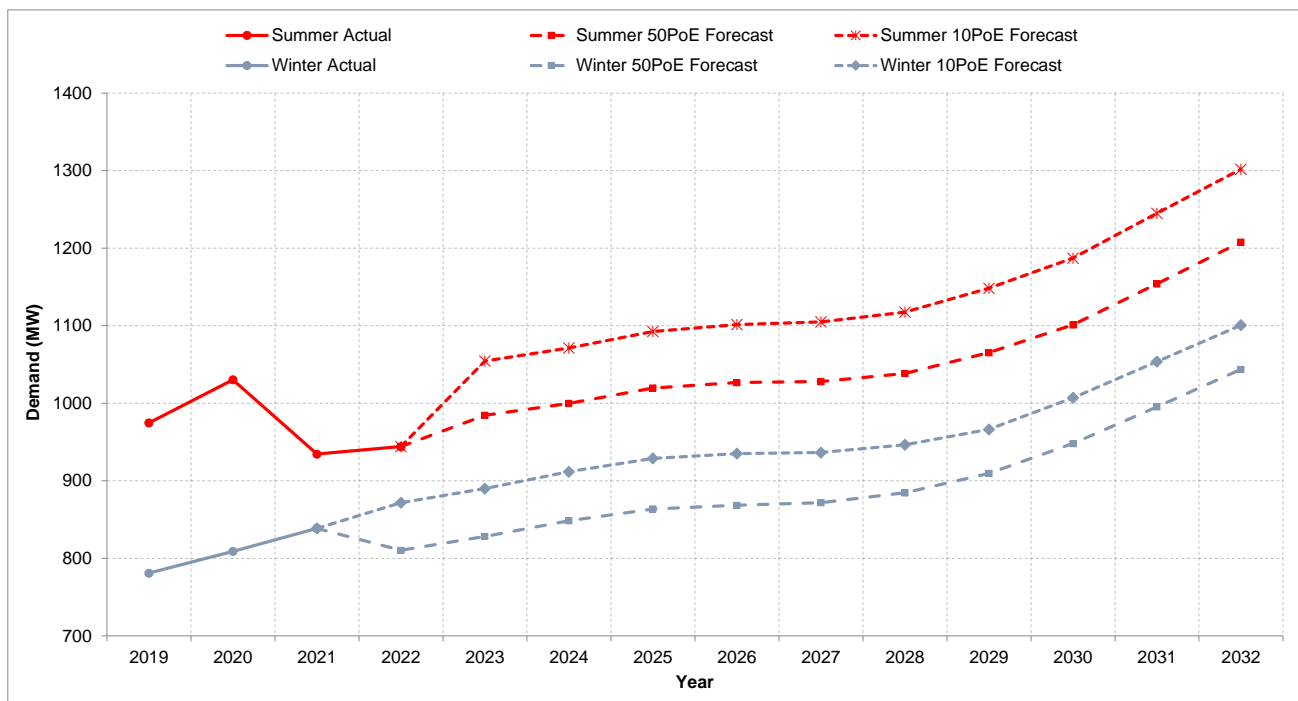
Figure 1: JEN historical and total maximum demand forecast
