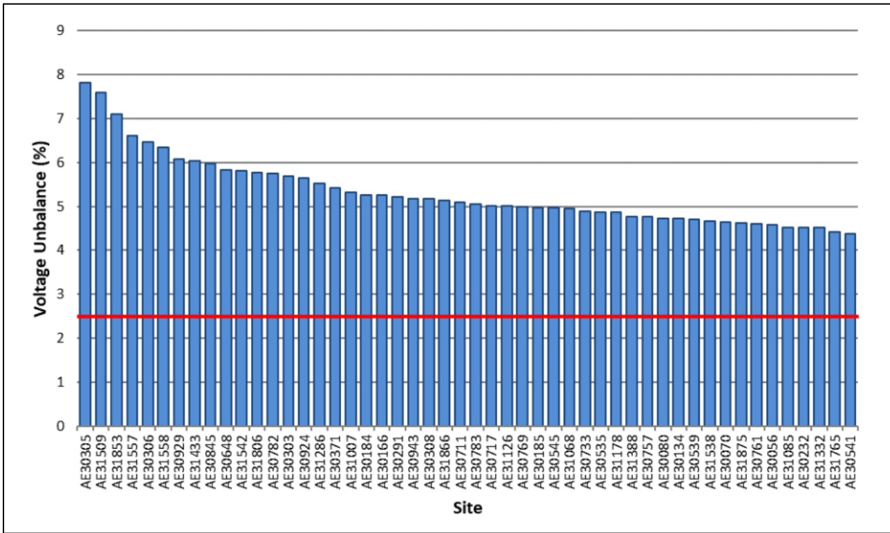
Figure 3-12: Voltage unbalance (negative sequence voltage) – LV sites (worst 50)
