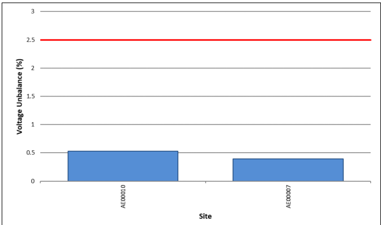
Figure 3-11: Voltage unbalance (negative sequence voltage) – 6.6 kV sites
