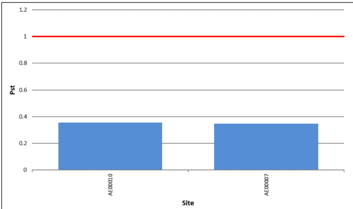
Figure 3-15: 6.6 kV Voltage flicker levels – Pst distribution
