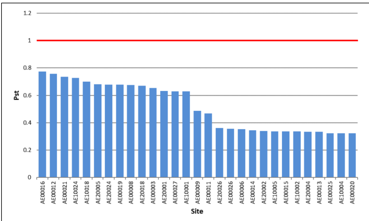
Figure 3-13: 11 kV and 22 kV Voltage flicker levels – Pst distribution
