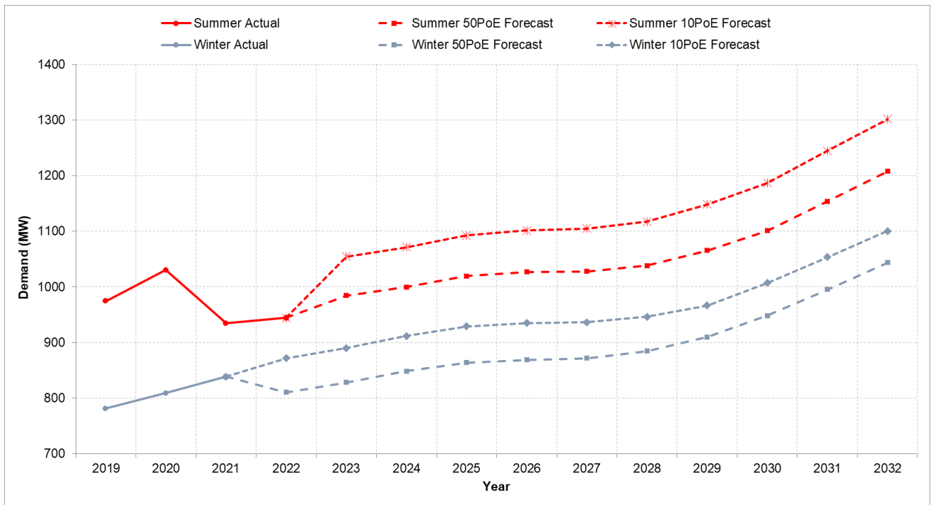
Figure 4-2: Jemena network historical and forecast maximum demand
