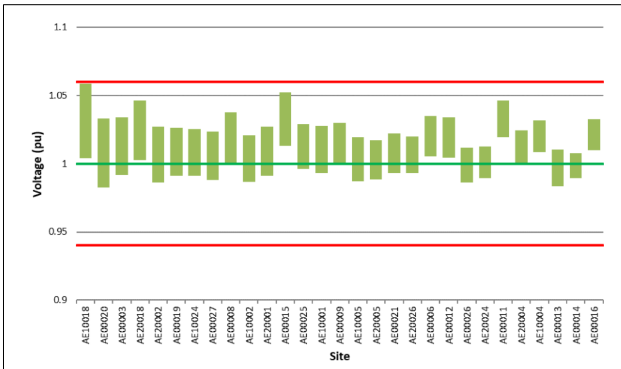
Figure 3-3: Steady-state voltage performance – 22 kV and 11 kV sites
