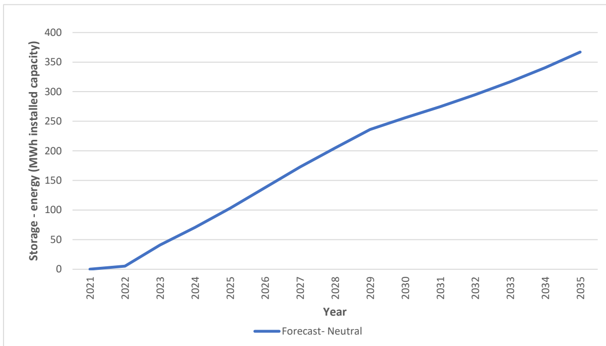
Figure 2-6: Forecast uptake of battery storage systems (MWh installed capacity) within Jemena’s supply area
