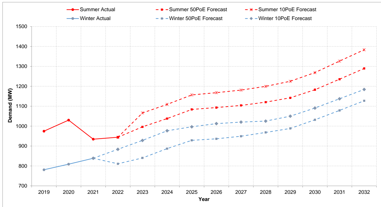
Figure 4-3: Forecast maximum demand with committed large customer connections
