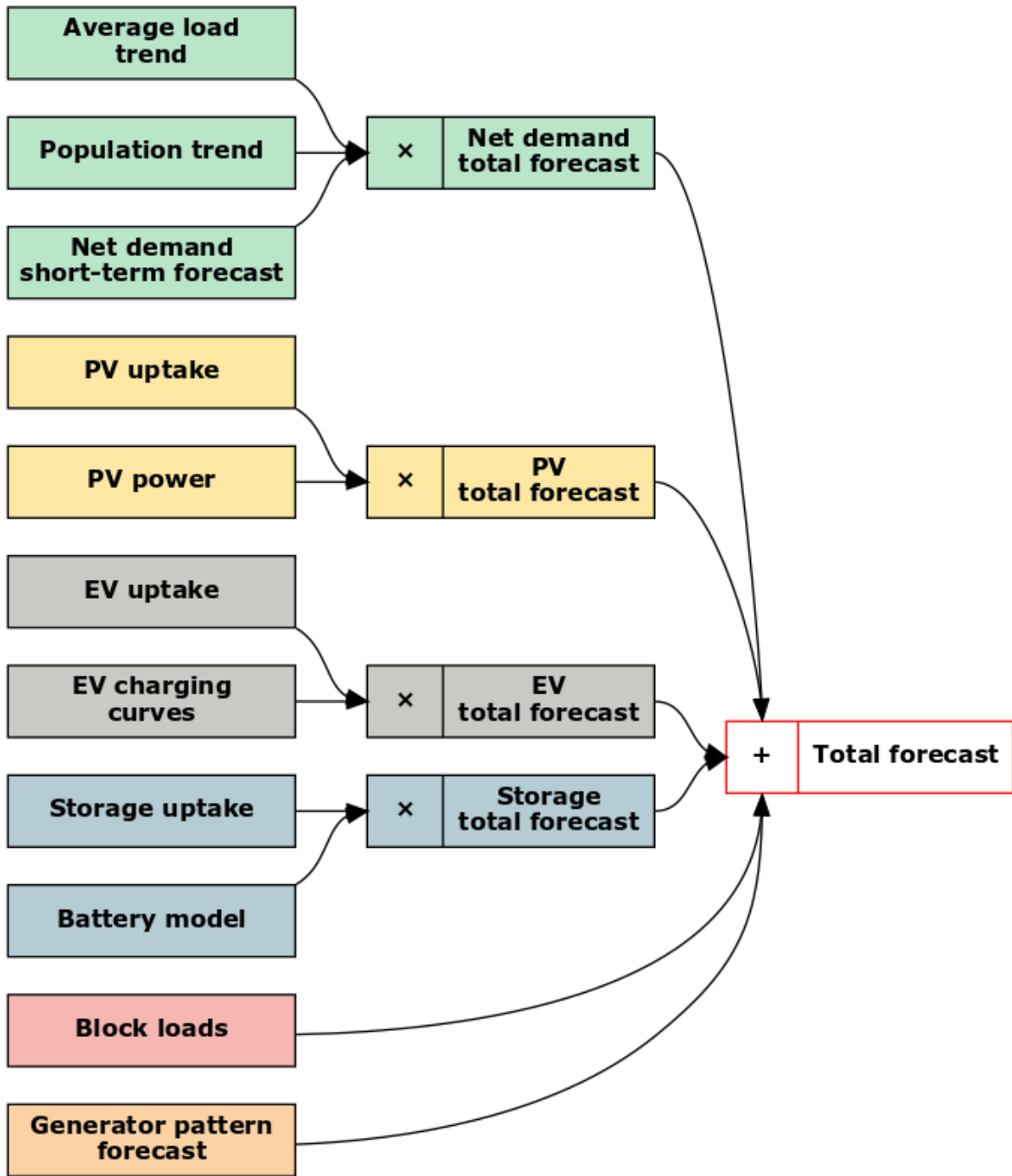
Figure 2-11: Overall process of aggregating the net demand forecast building blocks
