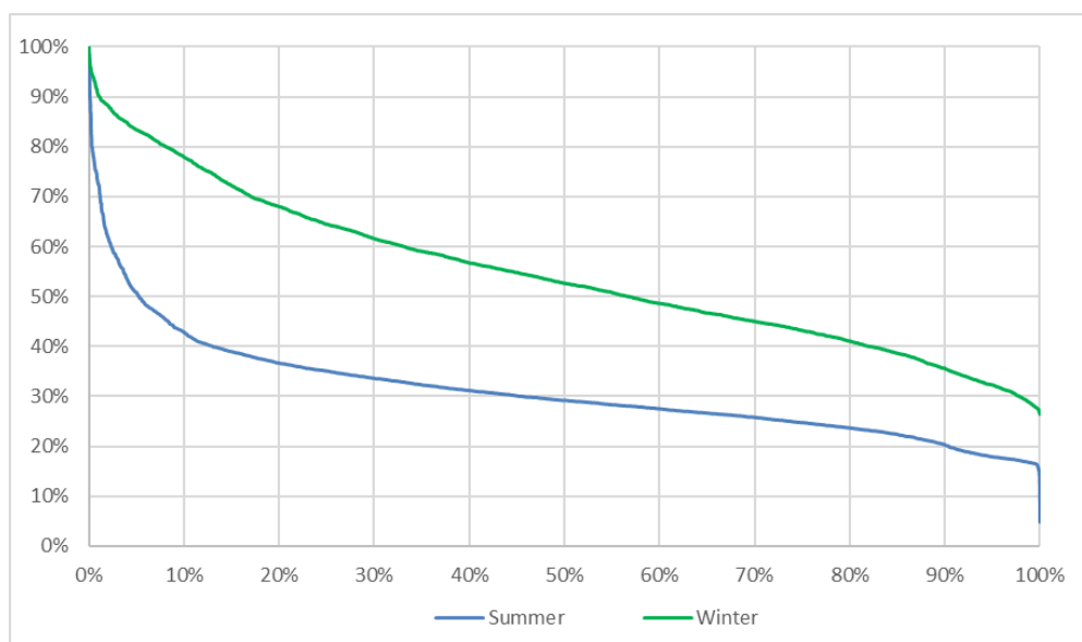
Figure 3–5: SHM load-duration curve (% of summer and winter maximum demand)
