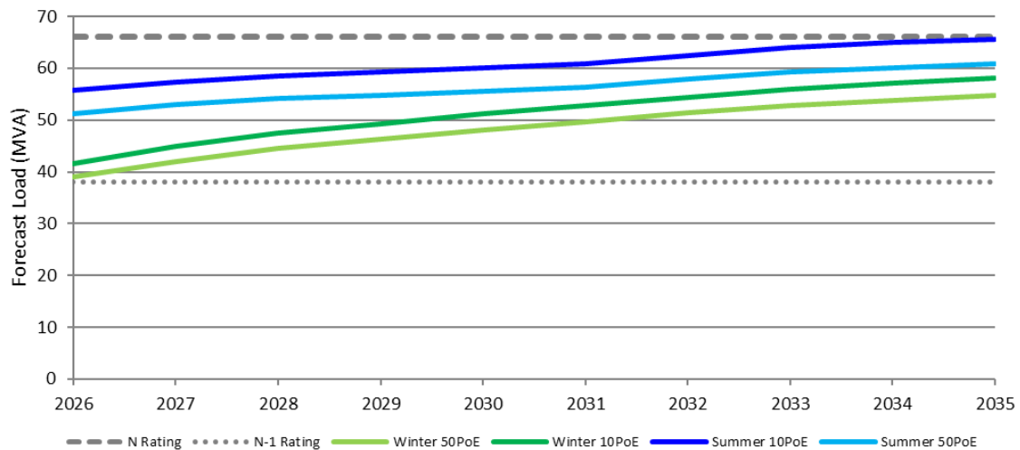
Figure 3–4: SHM maximum demand forecast and ratings (MVA)
