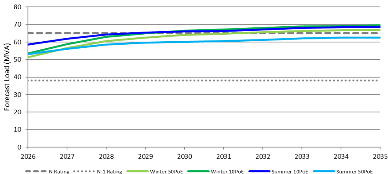
Figure 3–2: SBY maximum demand forecast and ratings (MVA)
