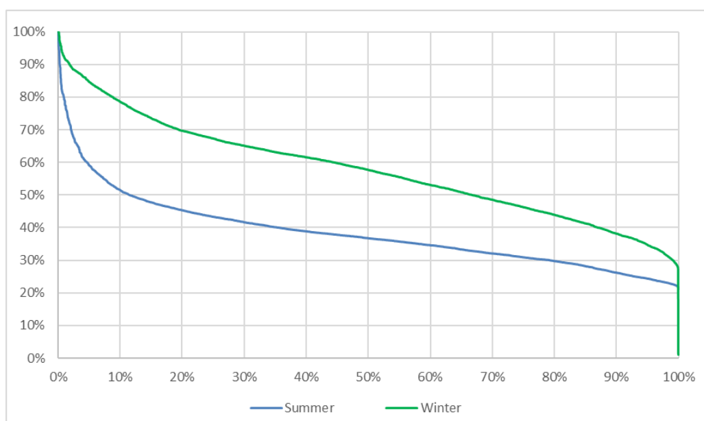
Figure 3–3: SBY load-duration curve (% of summer and winter maximum demand)
